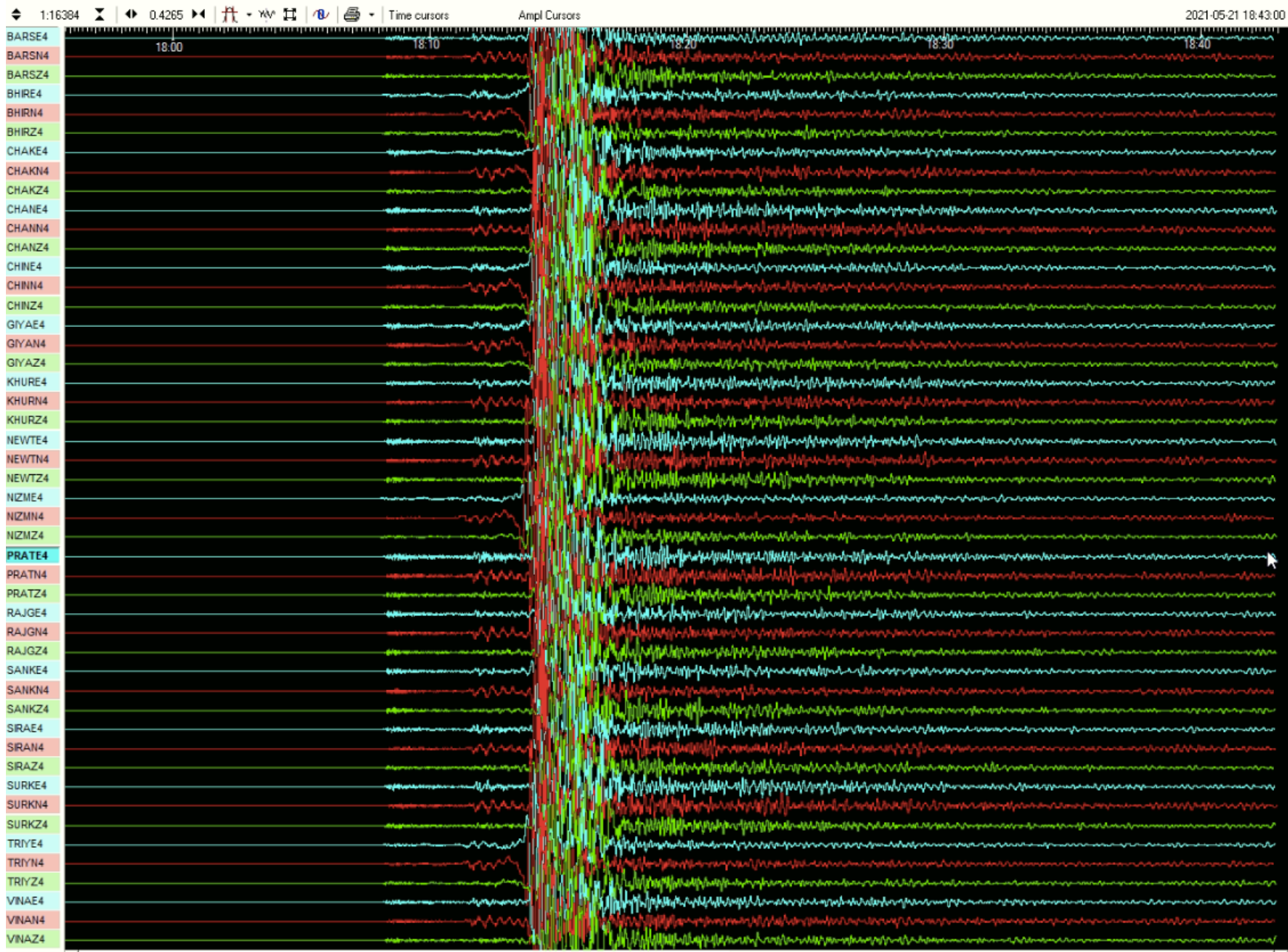
China earthquake of May 21, 2021 (Mag.- 7.0) occurred on 18:04:14 (UTC), 23:34:14 (IST), Lat., Long. : 34.65° N, 98.06° E, Focal Depth: 10 Km (as per NCS, New Delhi) recorded through VSAT based 18-stations Seismological Network around Tehri Region at Seismological Obs., IIT Roorkee.
